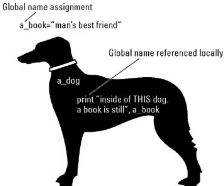
Figure 11-2: A global name referenced locally.
